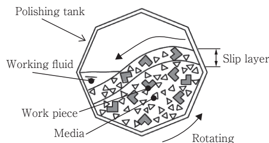
Fig. 1 Rotating barrel system
