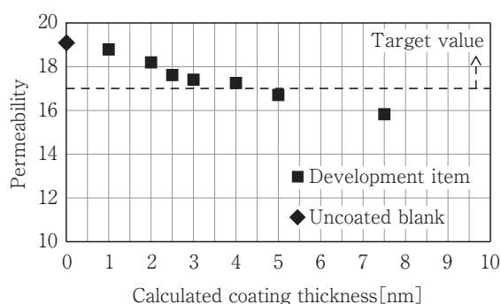
Fig. 4 Magnetic characteristic evaluation result.
