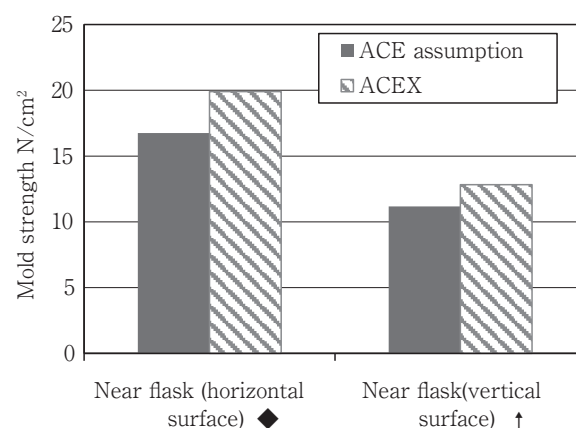
Fig. 12 Results of mold strength.
